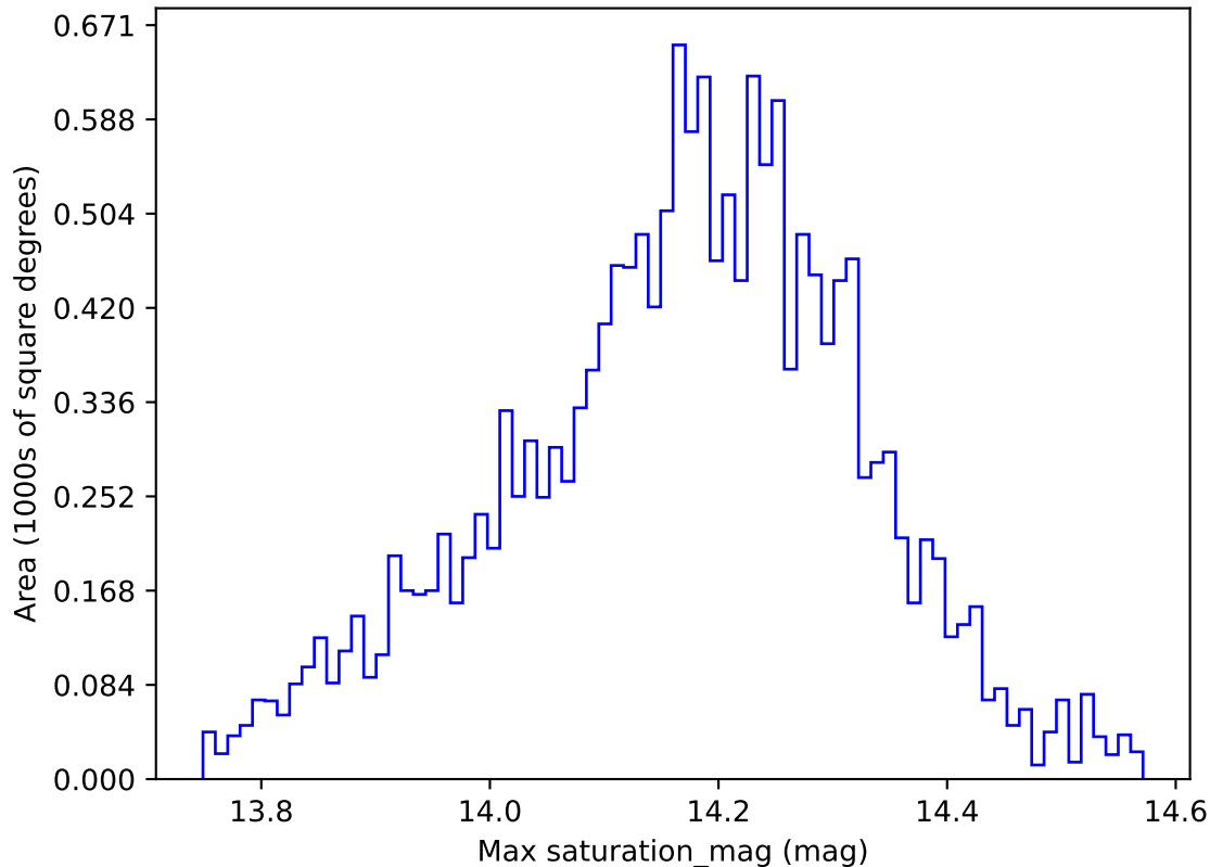
too_elab_r32_d3_giz_v3.4_10yrs WFD y band: Max saturation_mag
