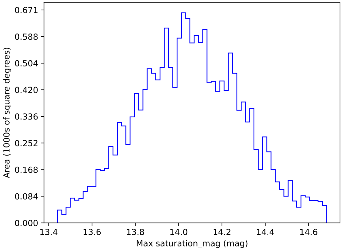
too_elab_r32_d3_giz_v3.4_10yrs WFD u band: Max saturation_mag
