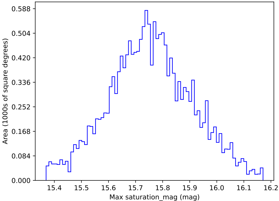
too_elab_r32_d3_giz_v3.4_10yrs WFD r band: Max saturation_mag
