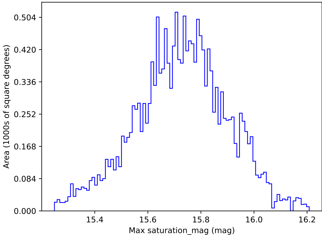
too_elab_r32_d3_giz_v3.4_10yrs WFD g band: Max saturation_mag
