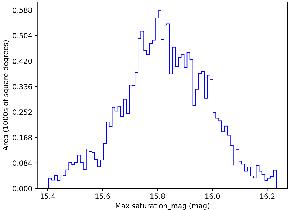
too_elab_r32_d3_giz_v3.4_10yrs WFD all bands: Max saturation_mag
