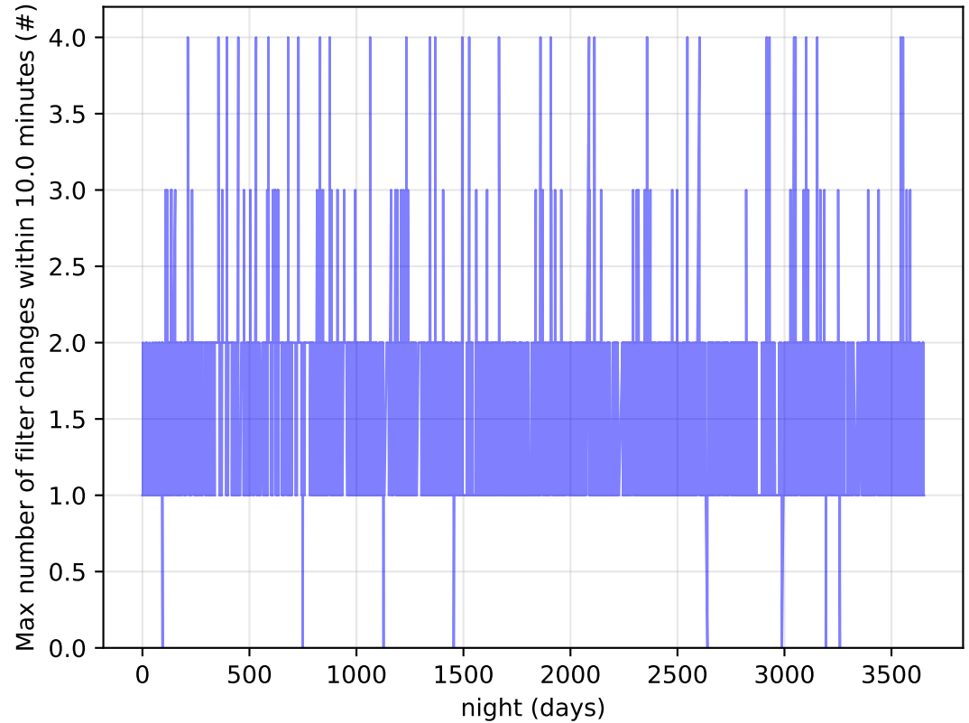
too_elab_r32_d3_giz_v3.4_10yrs Per Night: Max number of filter changes within 10.0 minutes
