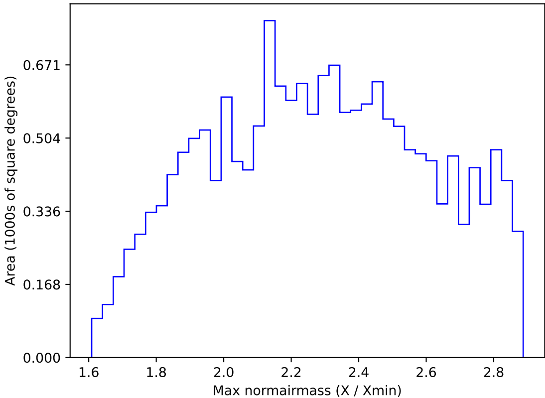
too_elab_r32_d3_giz_v3.4_10yrs WFD z band: Max normairmass
