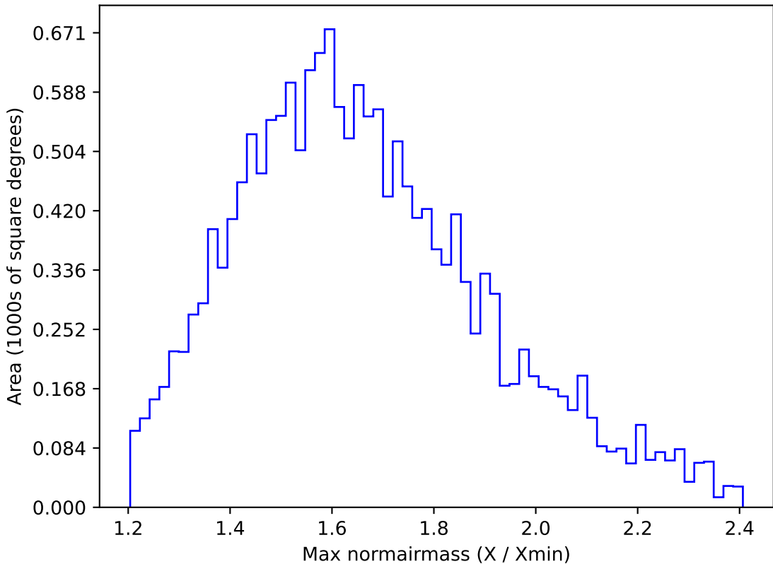
too_elab_r32_d3_giz_v3.4_10yrs WFD u band: Max normairmass
