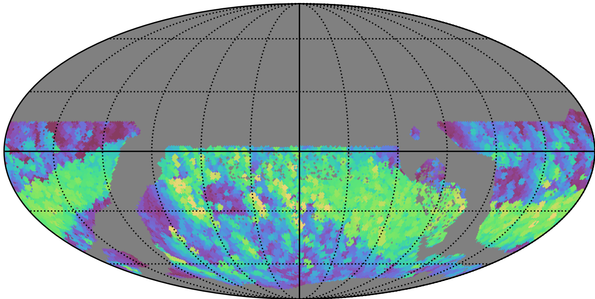
too_elab_r32_d3_giz_v3.4_10yrs WFD r band: Max normairmass
