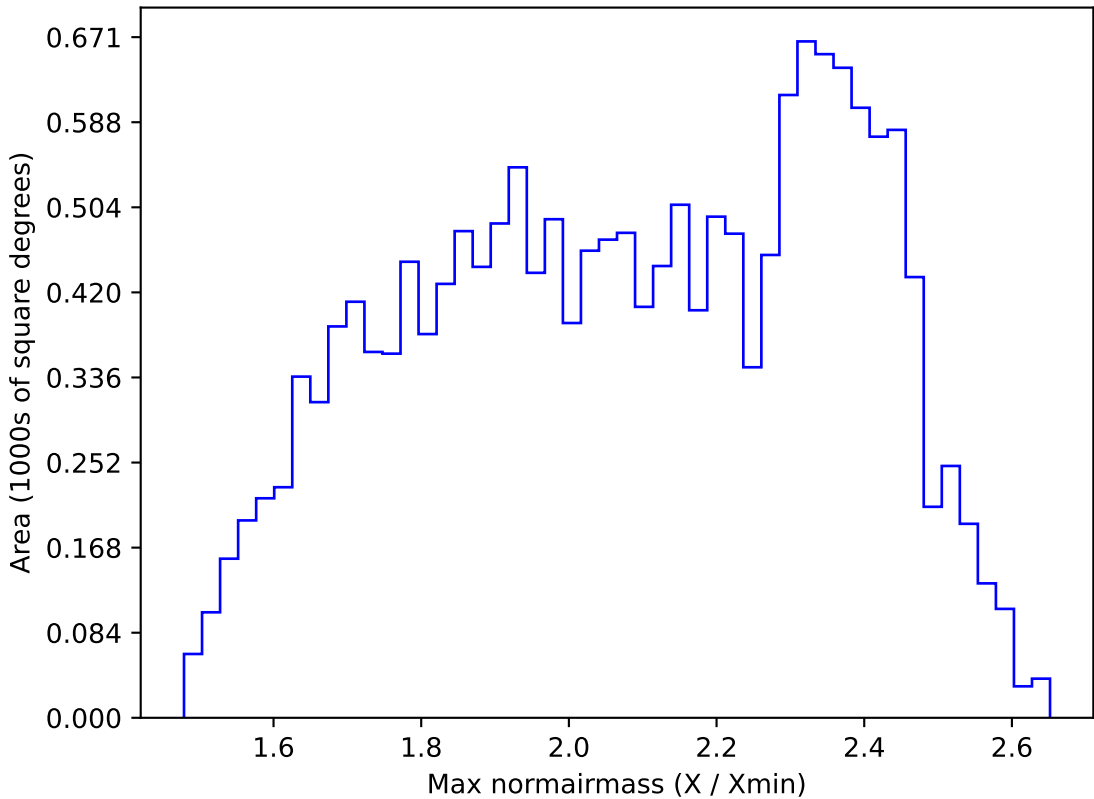
too_elab_r32_d3_giz_v3.4_10yrs WFD r band: Max normairmass
