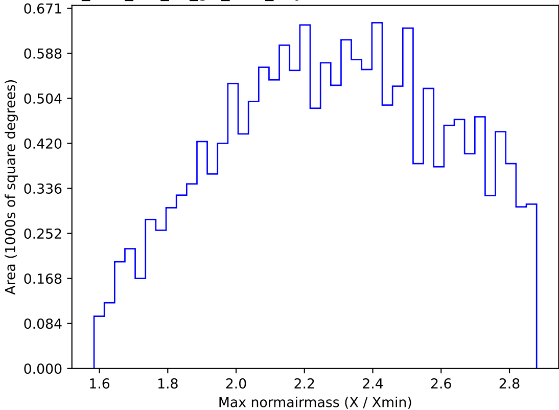
too_elab_r32_d3_giz_v3.4_10yrs WFD i band: Max normairmass
