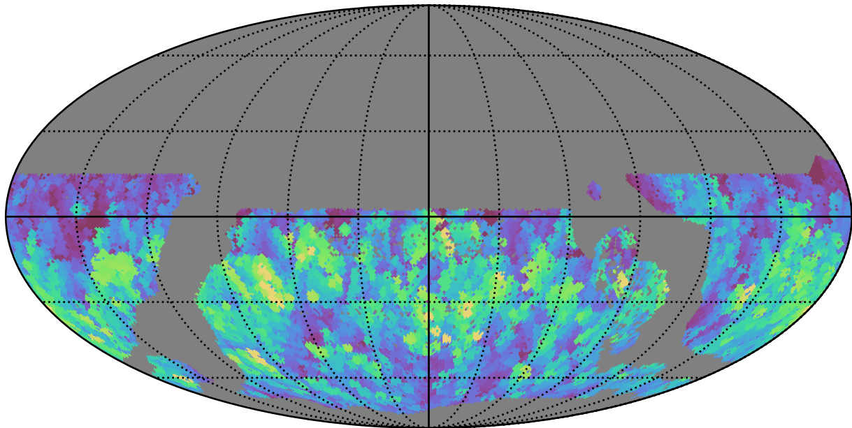
too_elab_r32_d3_giz_v3.4_10yrs WFD g band: Max normairmass
