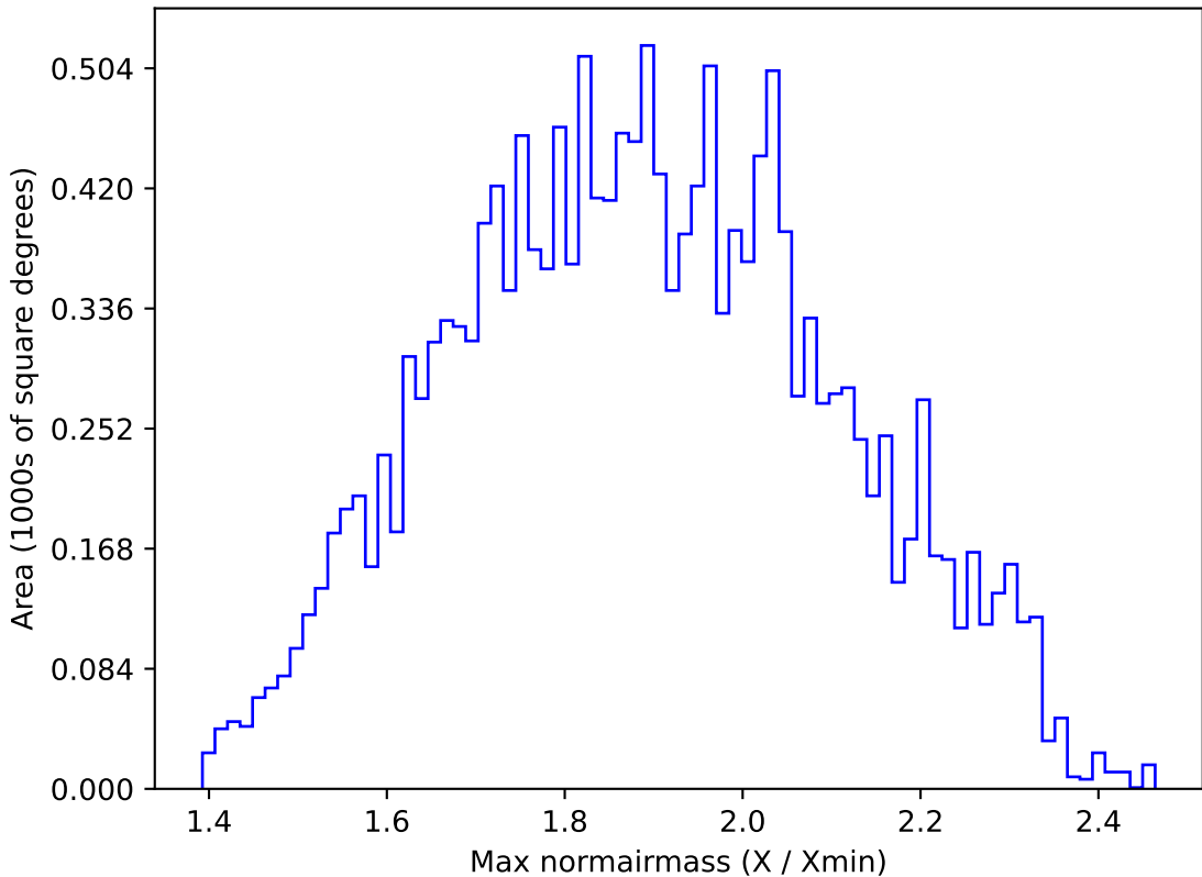
too_elab_r32_d3_giz_v3.4_10yrs WFD g band: Max normairmass
