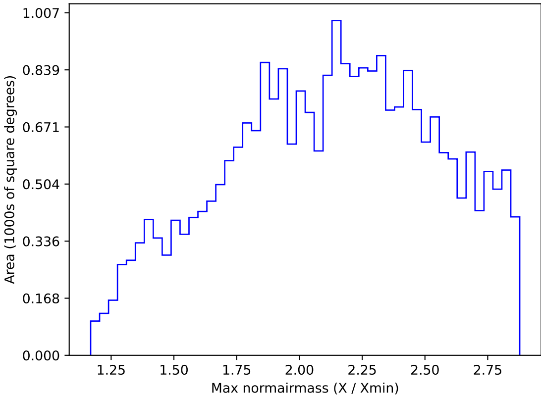
too_elab_r32_d3_giz_v3.4_10yrs All sky z band: Max normairmass
