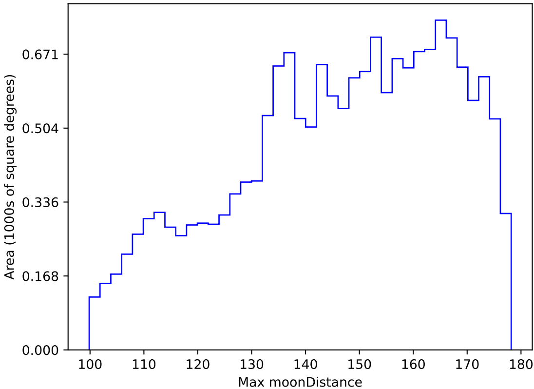
too_elab_r32_d3_giz_v3.4_10yrs WFD y band: Max moonDistance
