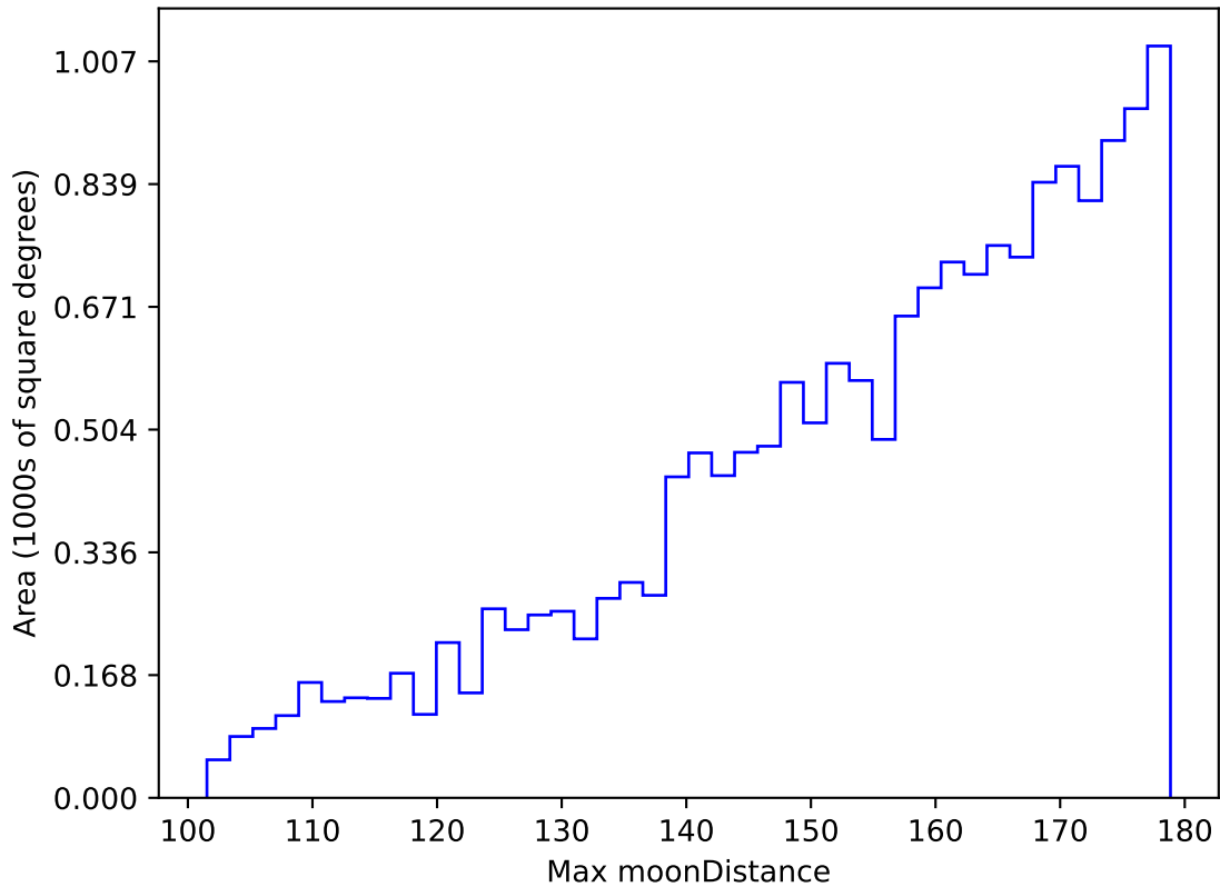
too_elab_r32_d3_giz_v3.4_10yrs WFD u band: Max moonDistance
