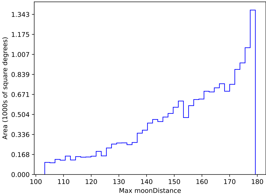
too_elab_r32_d3_giz_v3.4_10yrs WFD i band: Max moonDistance
