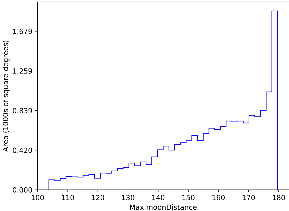
too_elab_r32_d3_giz_v3.4_10yrs WFD all bands: Max moonDistance
