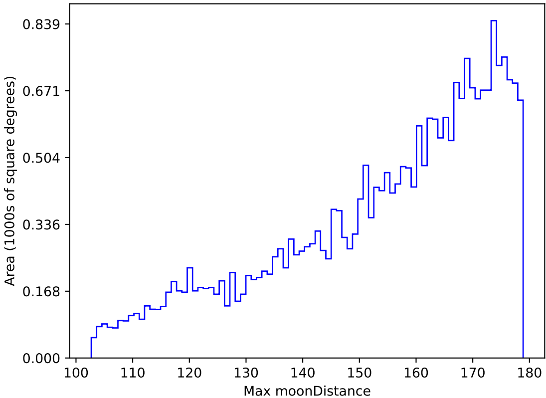
too_elab_r32_d3_giz_v3.4_10yrs All sky z band: Max moonDistance
