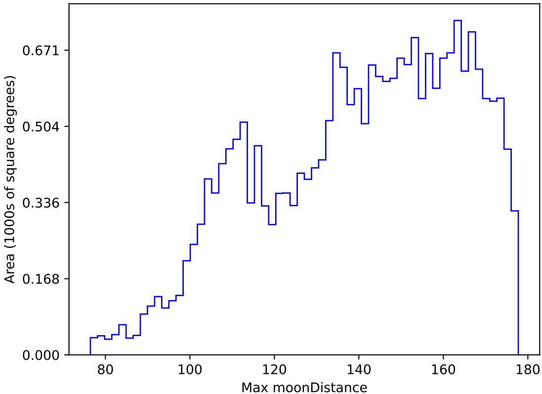
too_elab_r32_d3_giz_v3.4_10yrs All sky y band: Max moonDistance
