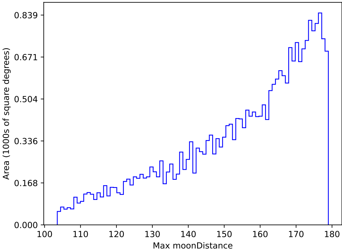
too_elab_r32_d3_giz_v3.4_10yrs All sky g band: Max moonDistance
