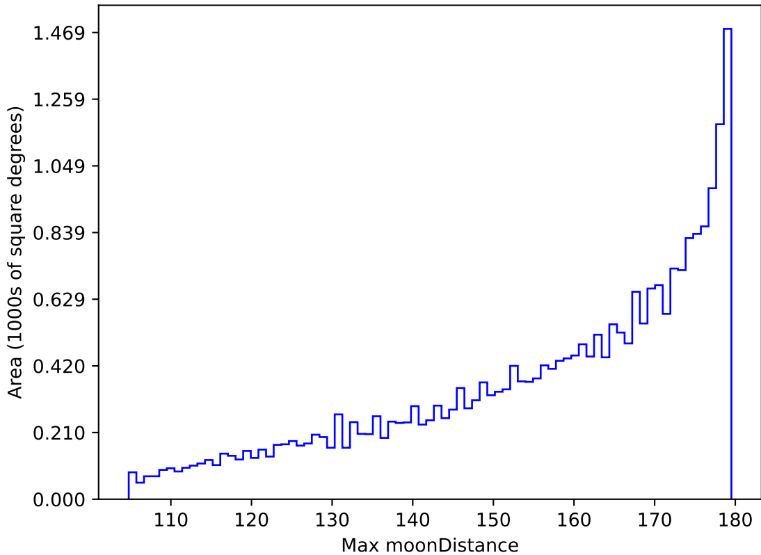
too_elab_r32_d3_giz_v3.4_10yrs All sky all bands: Max moonDistance
