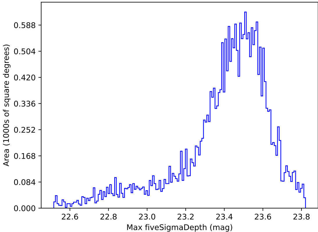
too_elab_r32_d3_giz_v3.4_10yrs Yr 1 z band: Max fiveSigmaDepth
