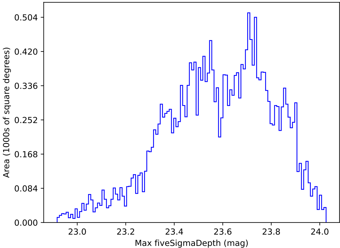
too_elab_r32_d3_giz_v3.4_10yrs Yr 1 u band: Max fiveSigmaDepth
