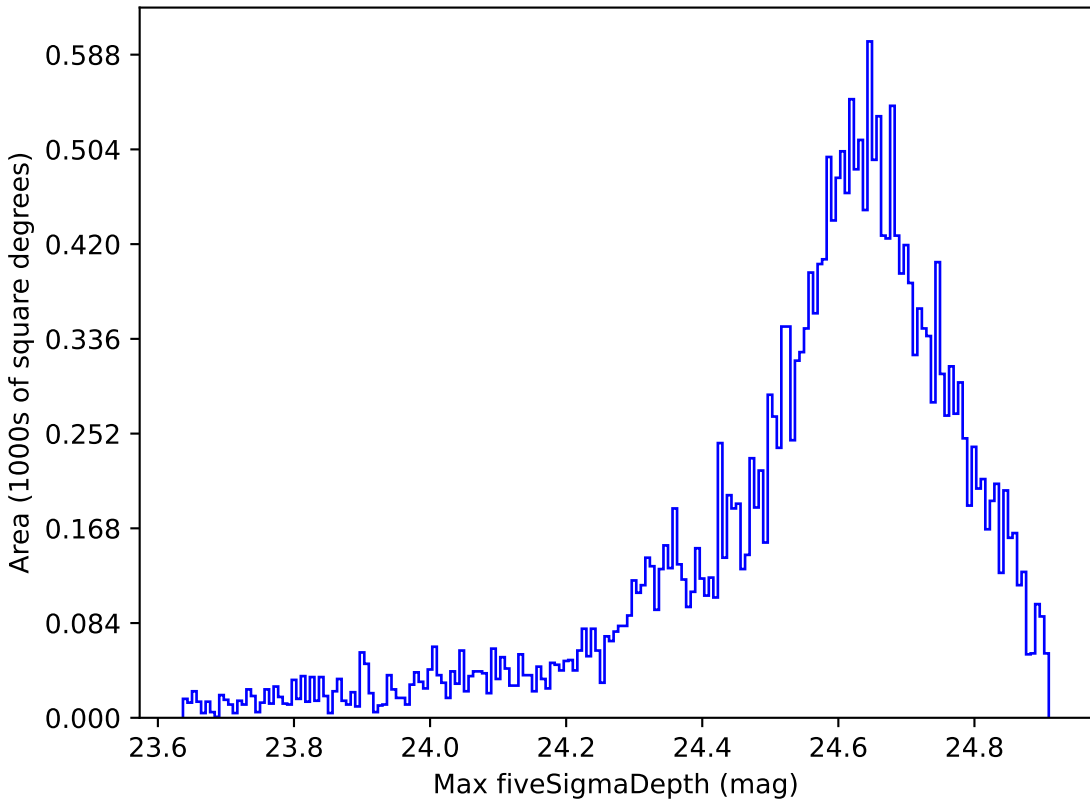
too_elab_r32_d3_giz_v3.4_10yrs Yr 1 r band: Max fiveSigmaDepth
