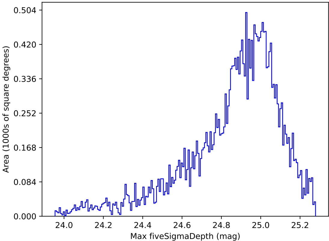
too_elab_r32_d3_giz_v3.4_10yrs Yr 1 g band: Max fiveSigmaDepth
