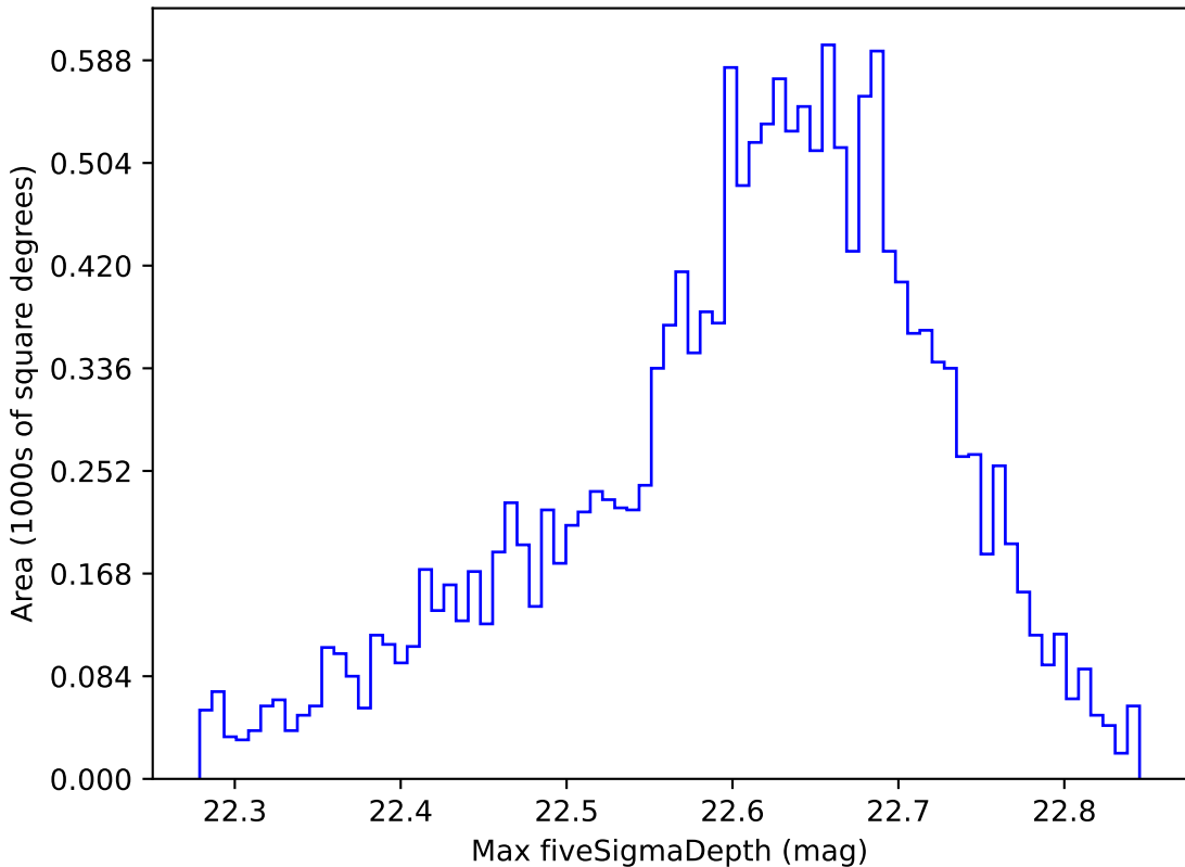
too_elab_r32_d3_giz_v3.4_10yrs WFD y band: Max fiveSigmaDepth
