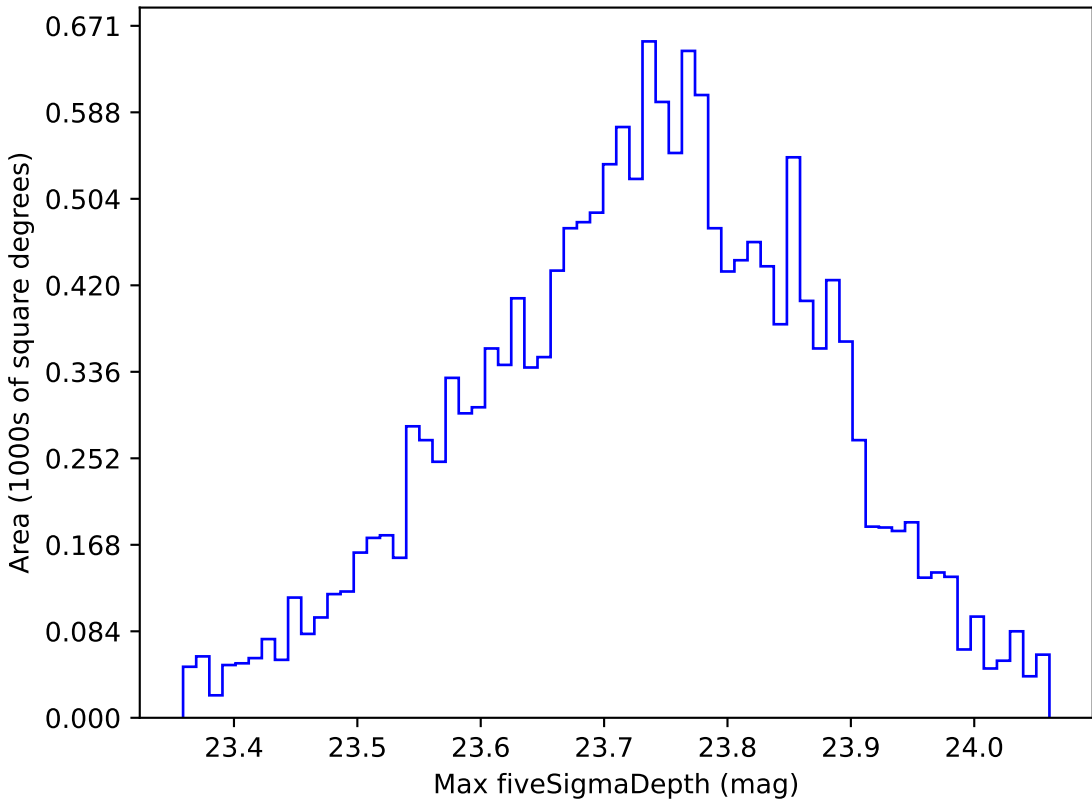
too_elab_r32_d3_giz_v3.4_10yrs WFD u band: Max fiveSigmaDepth
