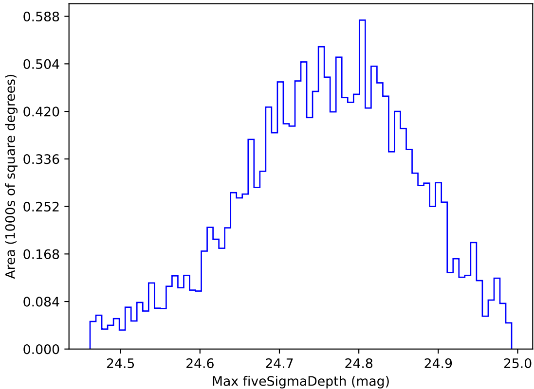
too_elab_r32_d3_giz_v3.4_10yrs WFD r band: Max fiveSigmaDepth
