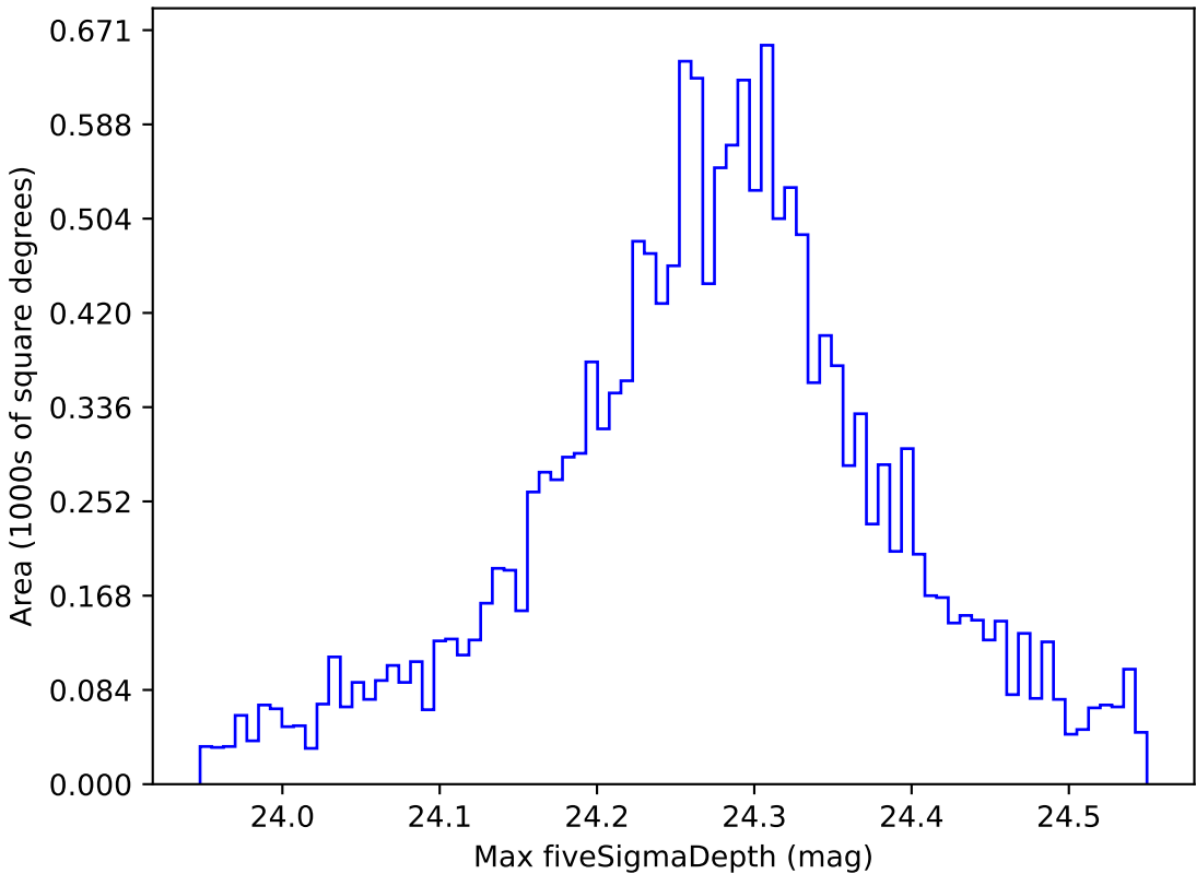
too_elab_r32_d3_giz_v3.4_10yrs WFD i band: Max fiveSigmaDepth
