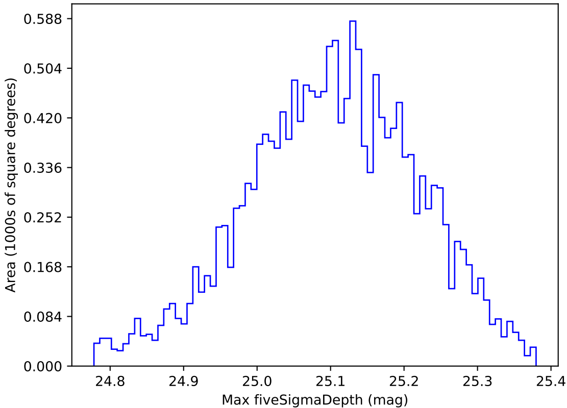
too_elab_r32_d3_giz_v3.4_10yrs WFD g band: Max fiveSigmaDepth
