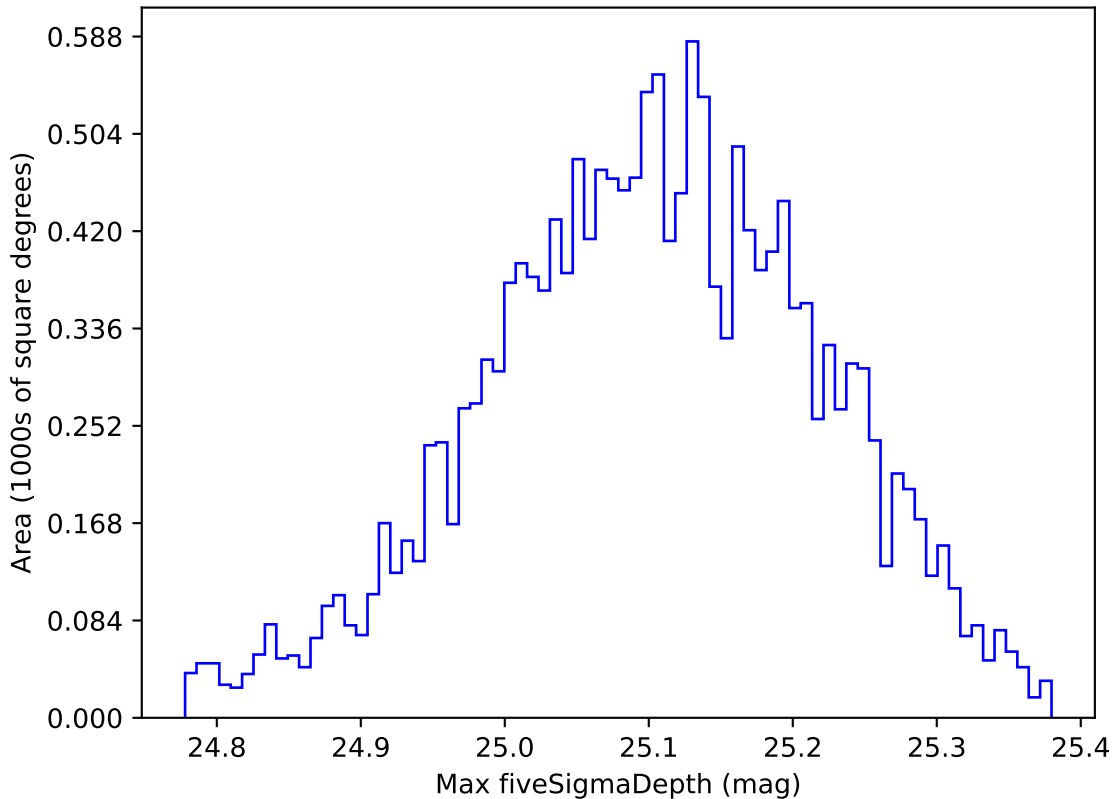
too_elab_r32_d3_giz_v3.4_10yrs WFD all bands: Max fiveSigmaDepth
