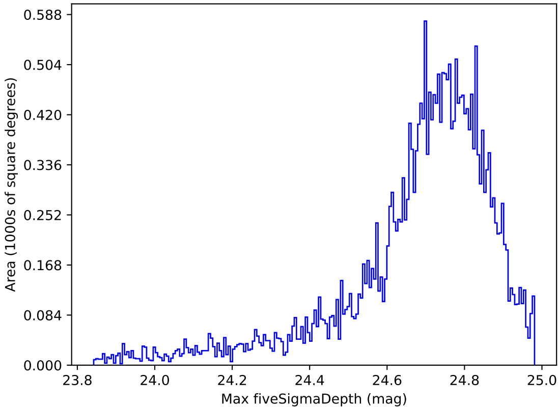
too_elab_r32_d3_giz_v3.4_10yrs All sky r band: Max fiveSigmaDepth
