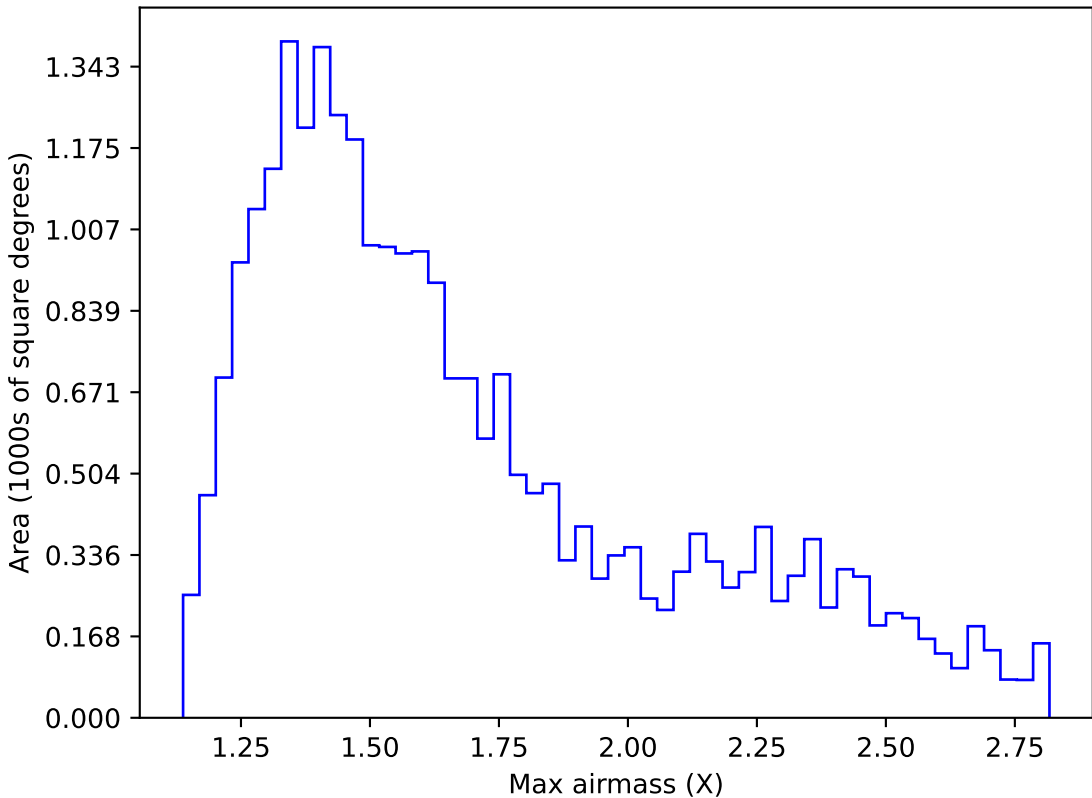
too_elab_r32_d3_giz_v3.4_10yrs Yr 1 z band: Max airmass
