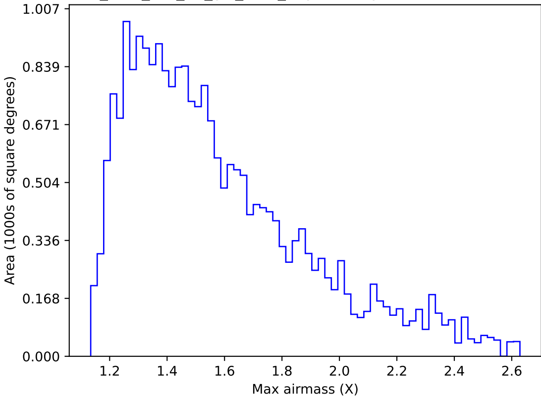
too_elab_r32_d3_giz_v3.4_10yrs Yr 1 y band: Max airmass
