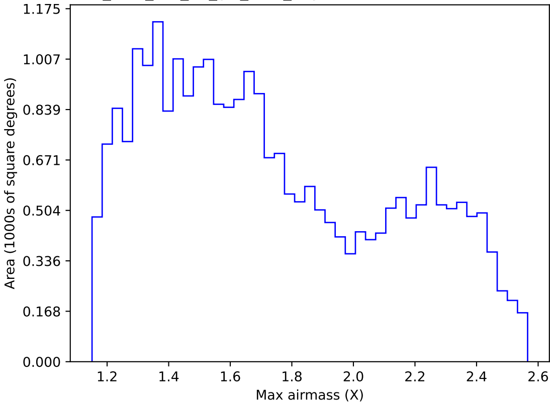
too_elab_r32_d3_giz_v3.4_10yrs Yr 1 r band: Max airmass
