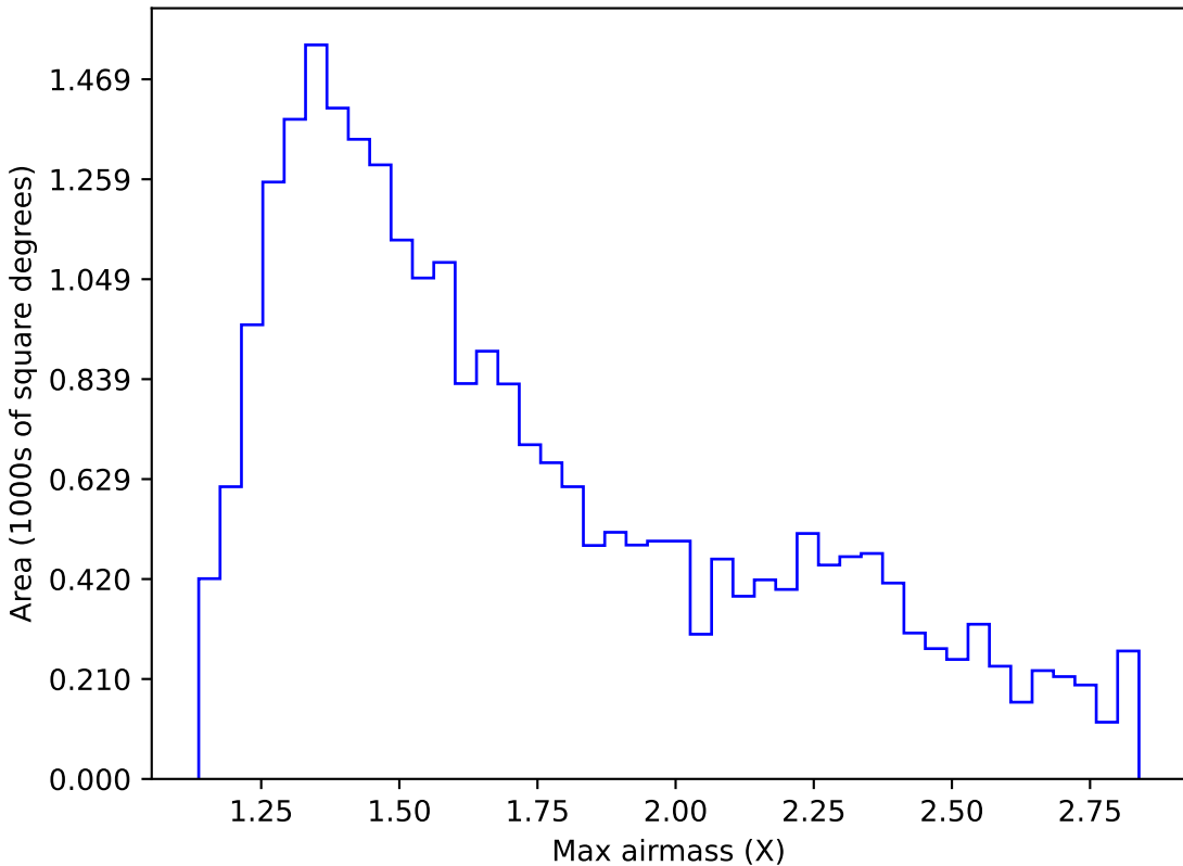
too_elab_r32_d3_giz_v3.4_10yrs Yr 1 i band: Max airmass
