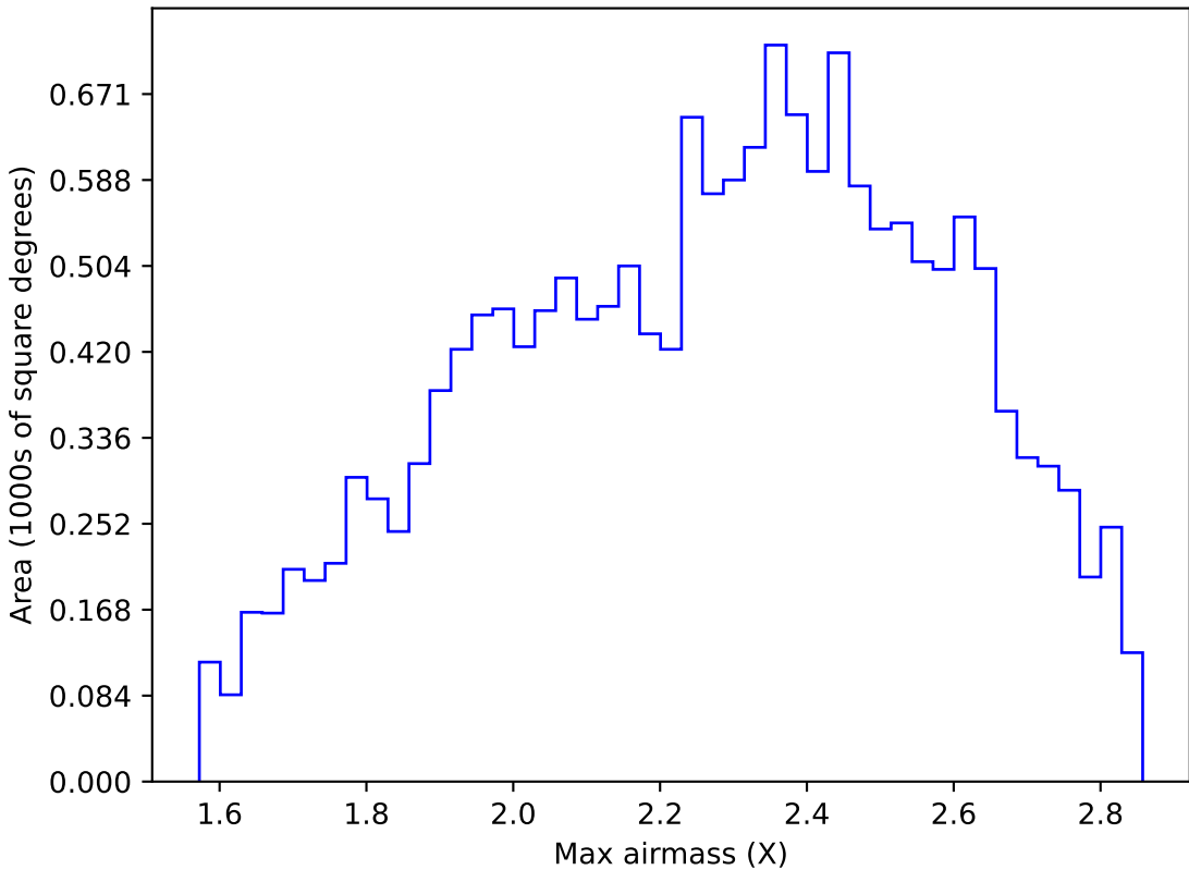
too_elab_r32_d3_giz_v3.4_10yrs WFD y band: Max airmass
