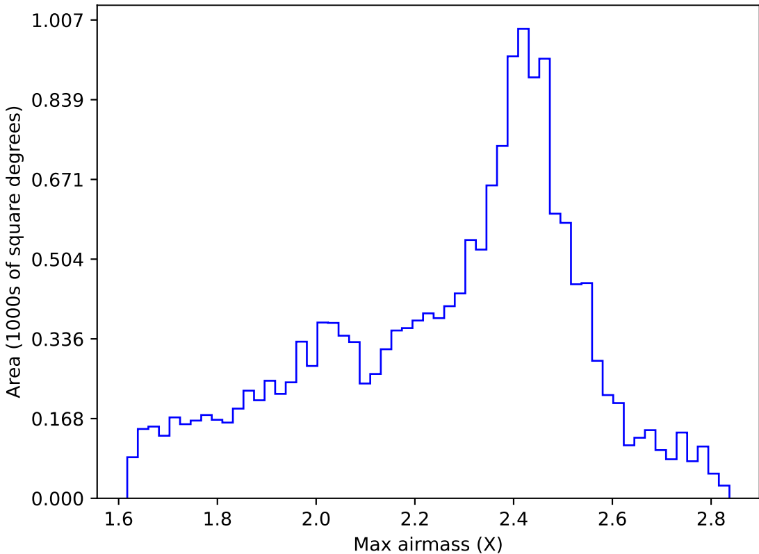
too_elab_r32_d3_giz_v3.4_10yrs WFD r band: Max airmass
