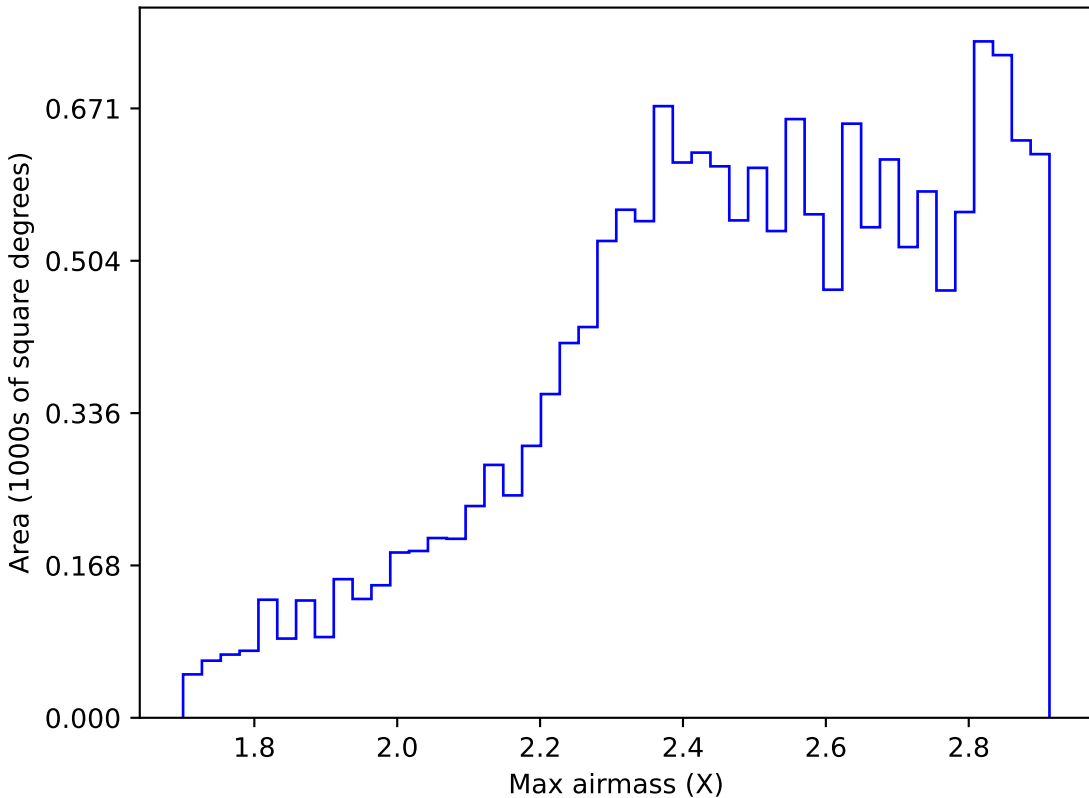
too_elab_r32_d3_giz_v3.4_10yrs WFD i band: Max airmass
