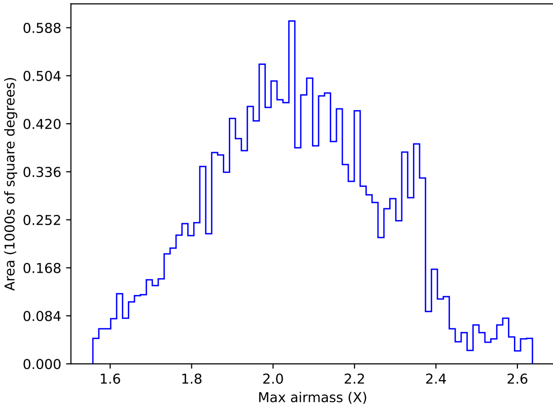
too_elab_r32_d3_giz_v3.4_10yrs WFD g band: Max airmass
