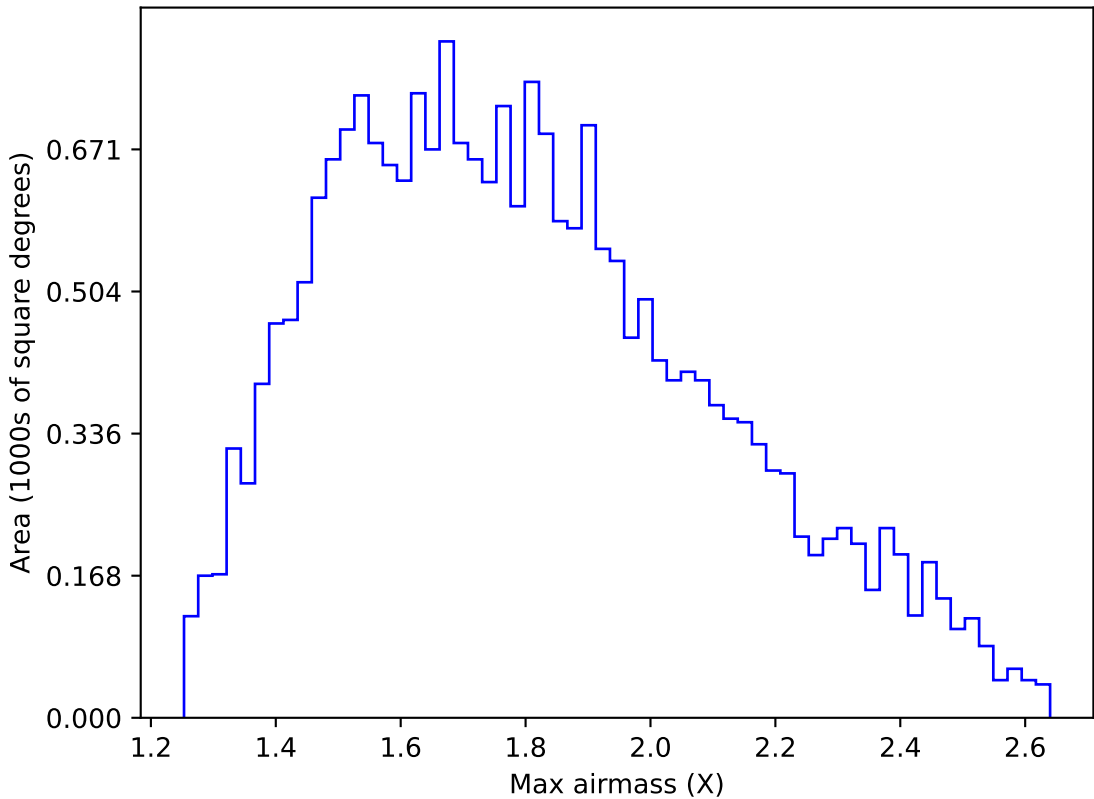
too_elab_r32_d3_giz_v3.4_10yrs All sky u band: Max airmass
