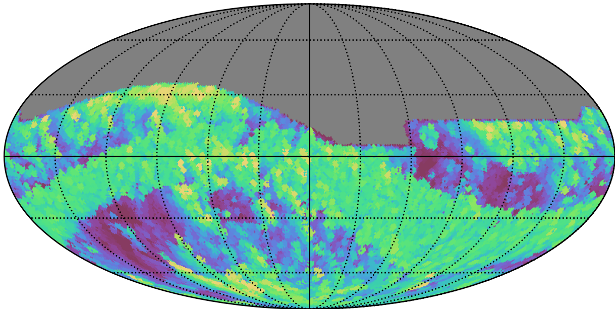
too_elab_r32_d3_giz_v3.4_10yrs All sky r band: Max airmass
