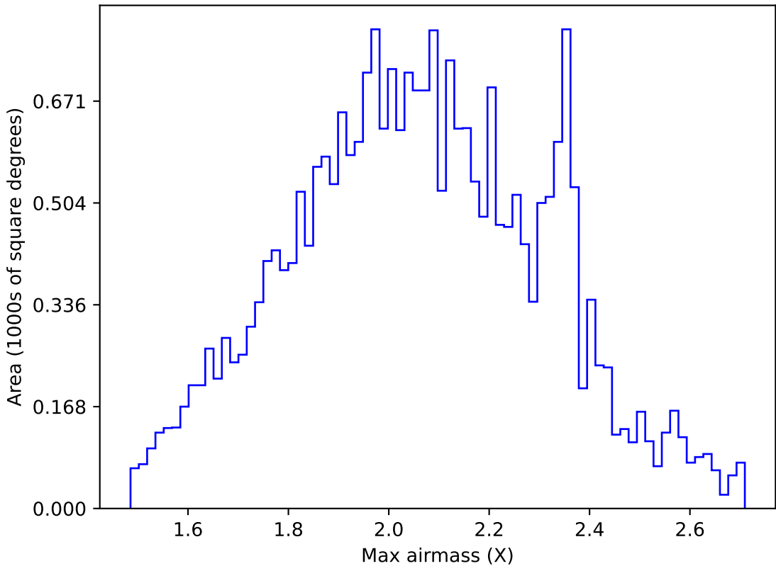
too_elab_r32_d3_giz_v3.4_10yrs All sky g band: Max airmass
