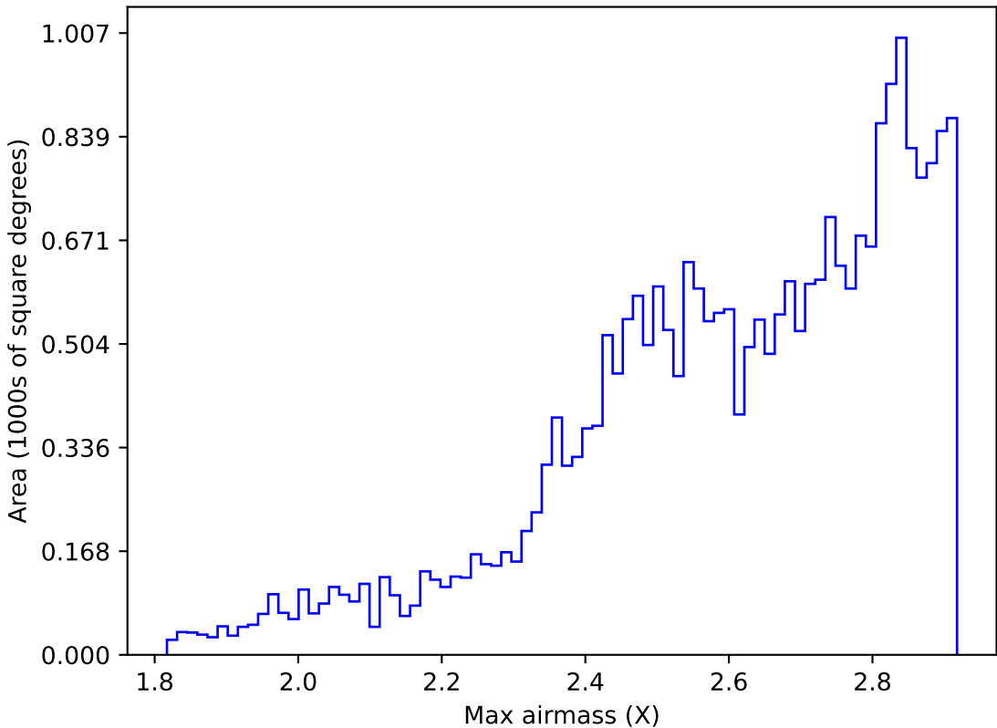
too_elab_r32_d3_giz_v3.4_10yrs All sky all bands: Max airmass
