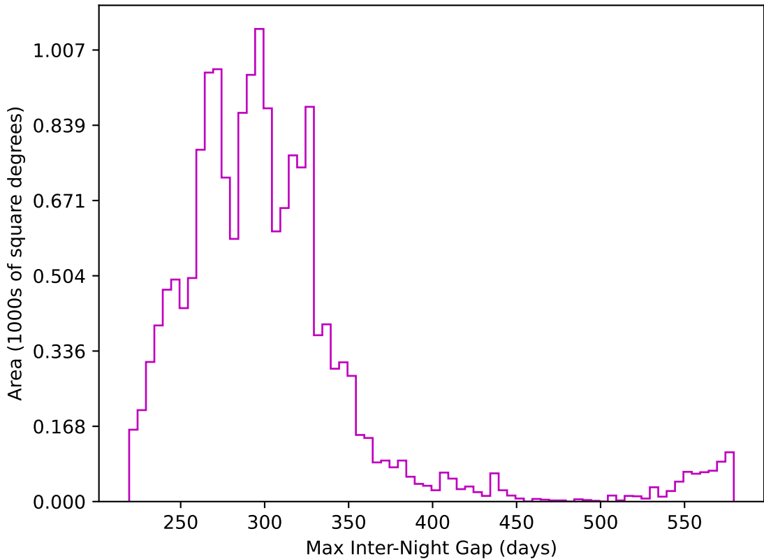
too_elab_r32_d3_giz_v3.4_10yrs WFD z band: Max Inter-Night Gap
