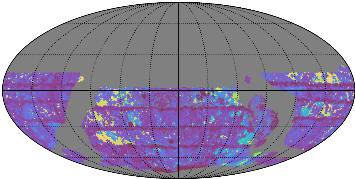
too_elab_r32_d3_giz_v3.4_10yrs WFD y band: Max Inter-Night Gap
