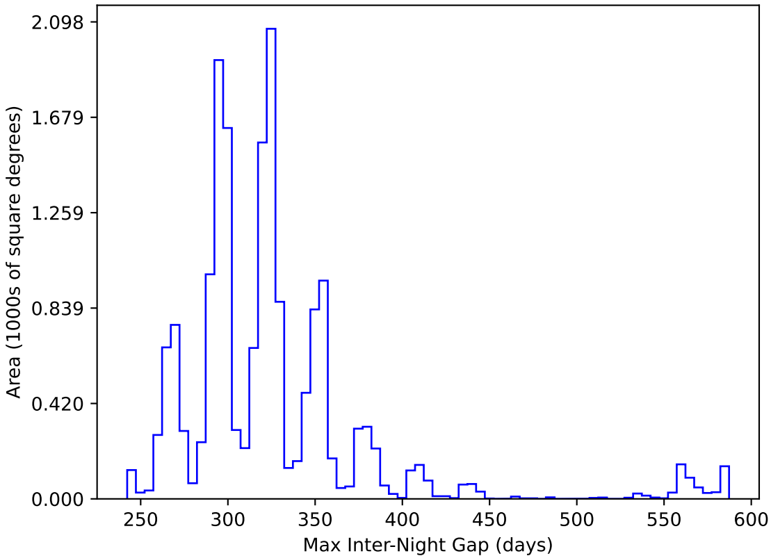
too_elab_r32_d3_giz_v3.4_10yrs WFD y band: Max Inter-Night Gap
