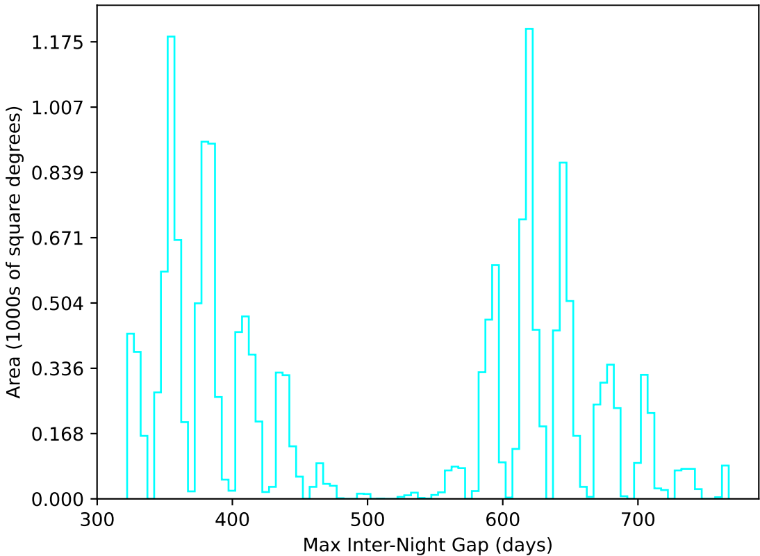
too_elab_r32_d3_giz_v3.4_10yrs WFD u band: Max Inter-Night Gap
