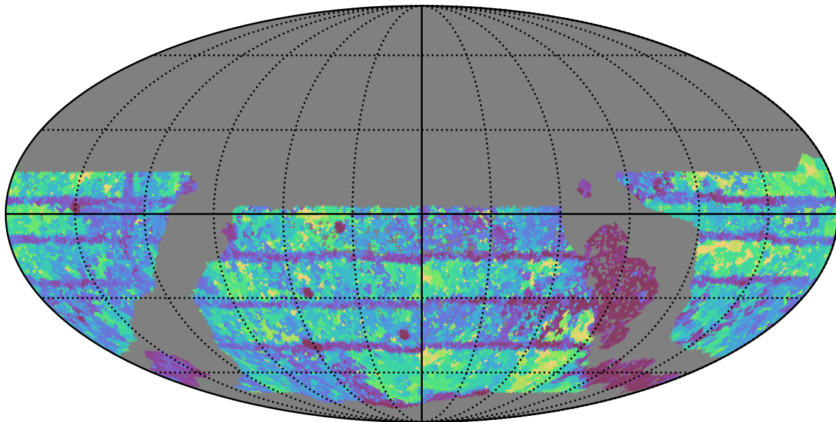
too_elab_r32_d3_giz_v3.4_10yrs WFD r band: Max Inter-Night Gap
